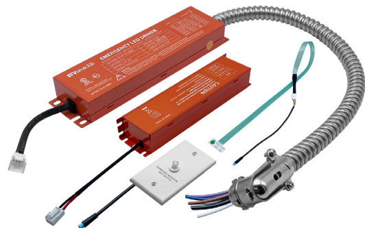
LED-EMB-25W-HV-2P
